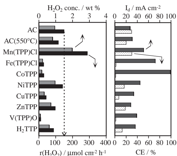
Figure 1. Electrocatalytic activities of metal-porphyrins supported on AC for the \text{H}_2\text{O}_2 formation by the \text{H}_2/\text{O}_2 fuel cell method at 25^\circ\text{C} .
