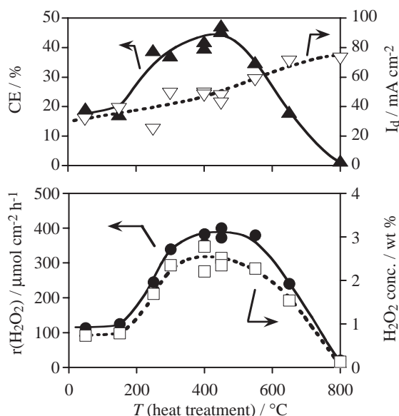
Figure 2. Effects of heat-treatment temperature of Mn(OEP)Cl/AC on the \text{H}_2\text{O}_2 formation by the \text{H}_2/\text{O}_2 fuel cell method at 25^\circ\text{C} .
